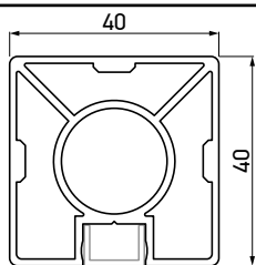
F40 Classic stub 40×40 mm - 6 m Antracit RAL 7016
